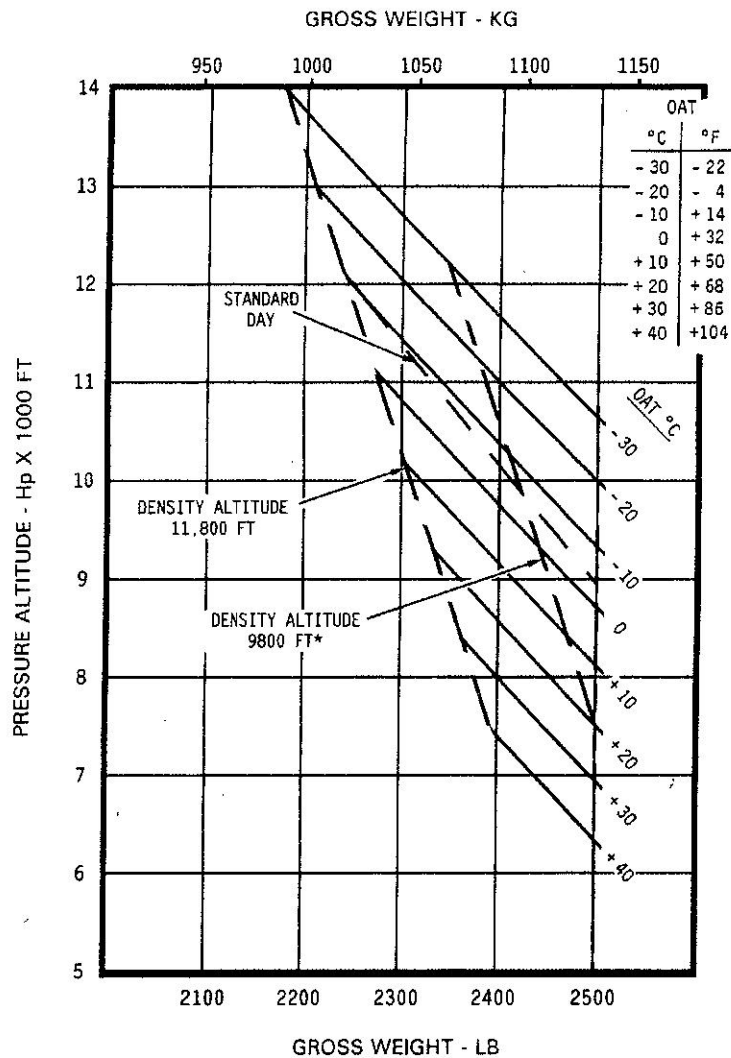
IGE HOVER CEILING VS. GROSS WEIGHT
